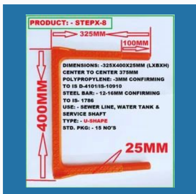
MANHOLE STEPS/RUNGS STEP X-8
