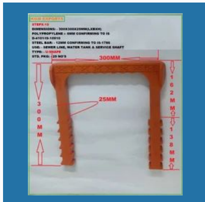
MANHOLE STEP/ RUNGS Step X-10
