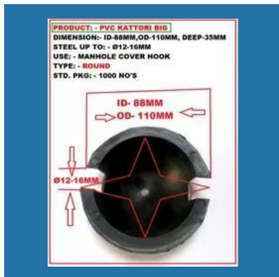
Pvc Kattori Round Cover
