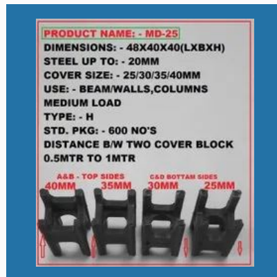
MD-25 Pvc Cover Blocks
